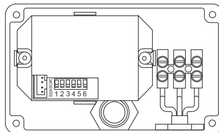
PIR Sensor Housing with cover removed
