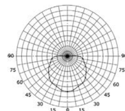
Ara canopy polar curve
